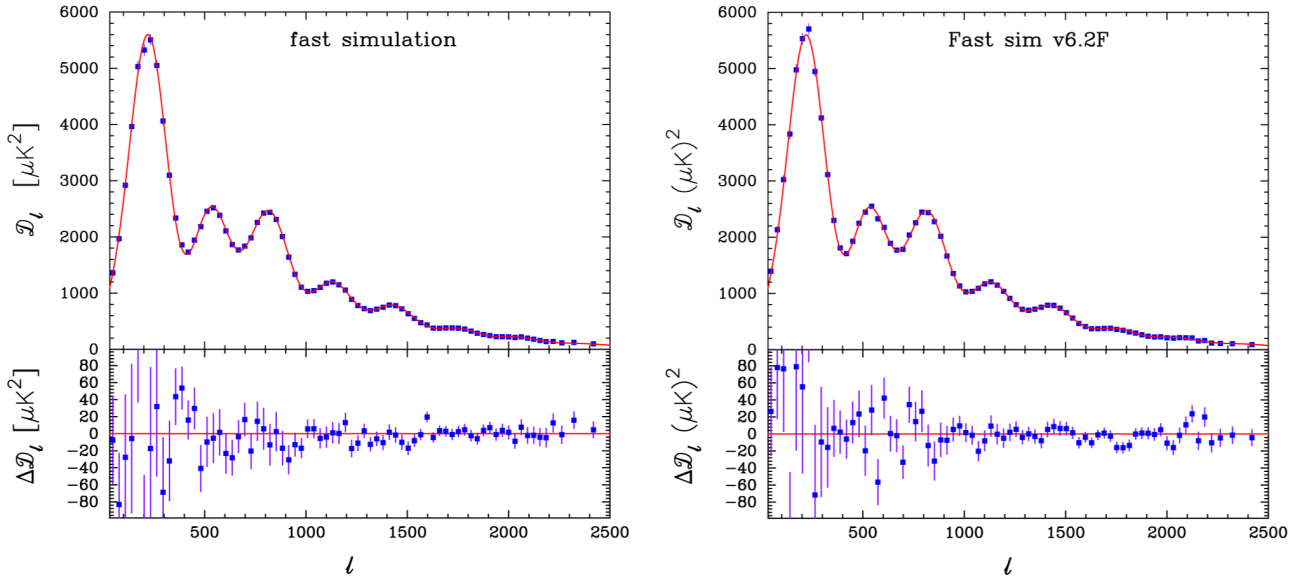
Fig. A.1. Toy power spectra drawn from a Gaussian distribution with mean given by a \Lambda CDM power spectrum and a covariance given by the band-averaged C_\ell covariance matrix, (top), and the corresponding differences with respect to the input \Lambda CDM model. Note the apparent presence of “coherent oscillatory features” in the difference spectra. These are fully described by the power spectrum covariance matrix. To assess the statistical significance of apparently “unexpected features” in the real spectrum, it is critical to include all sources of correlations among different C_\ell ’s.
